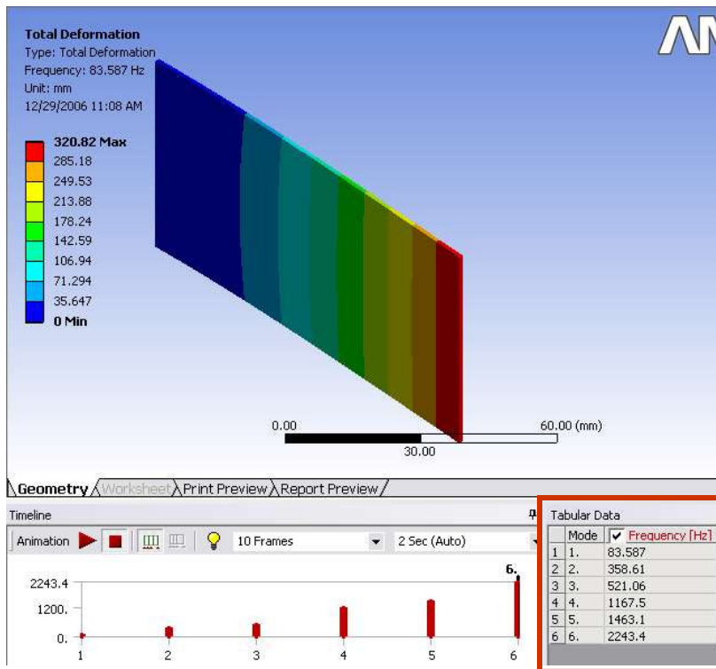
Free Vibration 1 st mode frequency: 83.587 Hz
