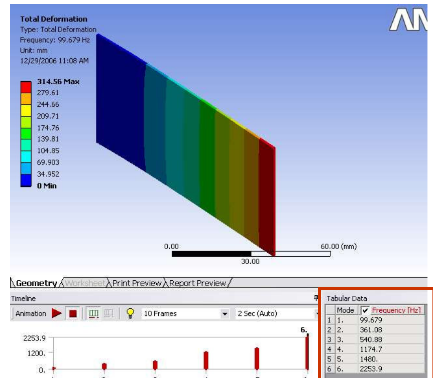
Free Vibration with Pre-Stress 1 st mode frequency: 99.679 Hz
